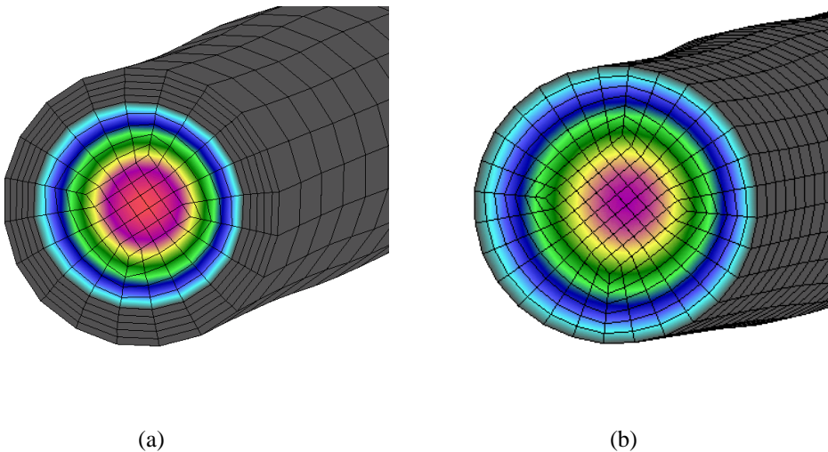
Fig. 1. Single layered and wall free model
