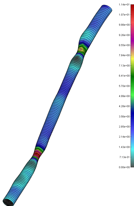
Fig. 2. Blood flow simulation – Shear stress distribution on the wall of the model generated from reconstructed IVUS medical images of rabbits carotid
